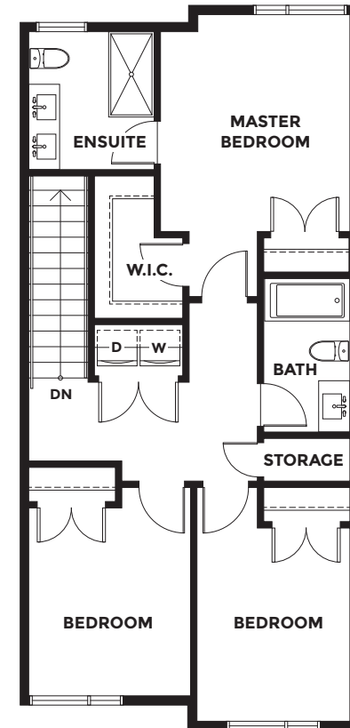
Upper Floor
