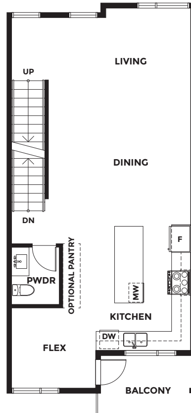
Main Floor
